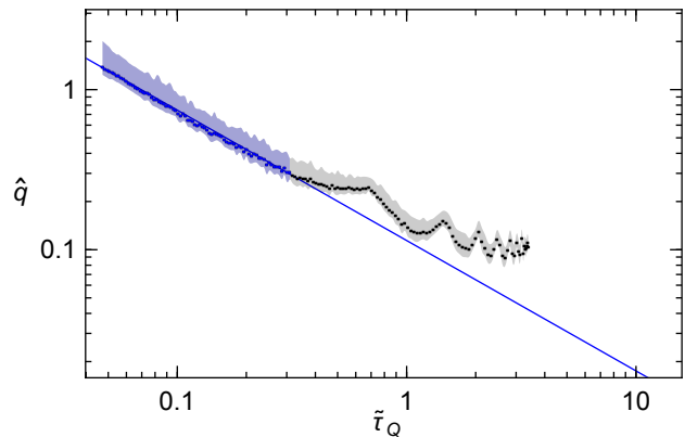
FIG. 11. Simulations including atoms loss. Similarly as in the experiment, the ramps begin at q = 1.1q_c and the initial number of atoms is 4 \times 10^4 atoms. Fits of the linear region (blue) with 0.05 < \bar{\tau}_Q < 0.31 give a scaling exponent of -0.80(3) .
