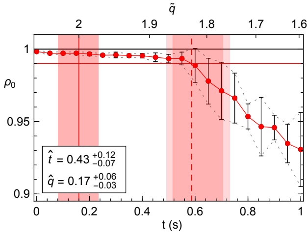
FIG. 25. t_r = 2.5 s, \tilde{\tau}_Q = 3.02 s
