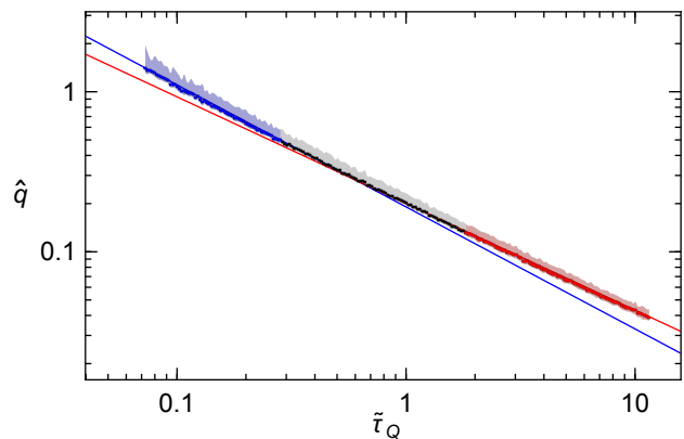
FIG. 7. Simulations in ideal conditions. The ramps start from 8.7|c| (1 G), which is much higher than the critical point, as compared to the experiment. A fit of the faster ramps (blue) with 0.05 < \tilde{\tau}_Q < 0.28 gives a scaling exponents of -0.76(5) . The slowest ramps (red) with \tilde{\tau}_Q > 1.83 yield scaling exponents of -0.67(2) .
