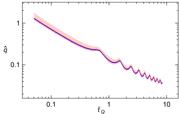
FIG. 12. Comparison of semi-classical and quantum simulations. The outputs from loss-less semi-classical and quantum simulations for 4 \times 10^4 atoms are compared. The ramps start at 500 mG, with a critical magnetic field set at B_c = 480 mG, which explains the oscillations for longer ramps. The solid red line is the output of the quantum simulation, and the shaded region represents one standard deviation. The blue dots show the output of the semi-classical simulation, performed with 1000 samples.
