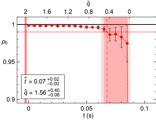
FIG. 13. t_r = 0.1 s, \tilde{\tau}_Q = 0.05 s
